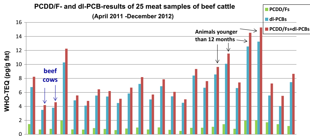
Fig. 3 PCDD/F and dl-PCB TEQ levels in meat of beef cattle on a pasture with elevated PCB-soil levels (mean 2 ng WHO-PCB-TEQ/kg dm, range 0.7–5.6) [29]
