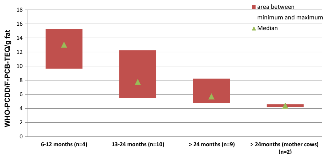
Fig. 4 TEQ levels in meat of cattle within one suckler cowherd in relation to age at slaughter [29, 52]
