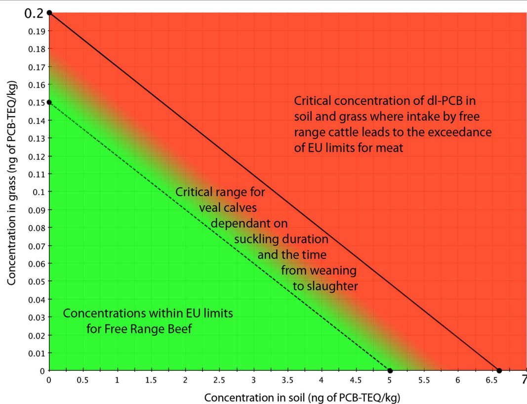
Fig. 2 Cumulative impact of grass and soil contaminated with dl-PCBs on exceedance of EU maximum levels for the sum of dioxins and dl-PCBs in beef and veal from suckling calves. Concentrations above the solid line are critical for beef and concentrations above the dashed line are critical for veal from suckling calves [17]
