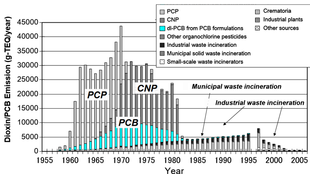
Fig. 6 Historic release of PCDD/Fs into the environment of Japan [295, 130]
